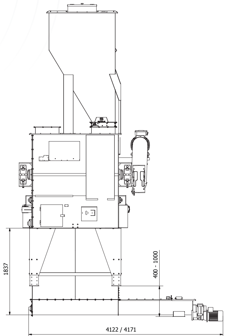
Dimensions in mm for PTS2000 / PTS4000
